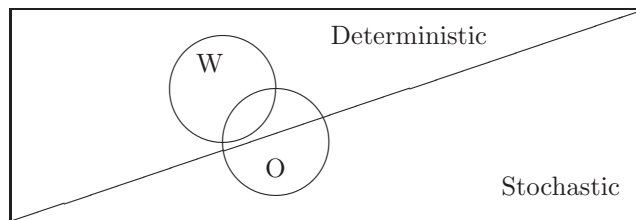
FIG. 1. NP-hard optimization problems and the frameworks of Woeginger (W) and of ours (O).
