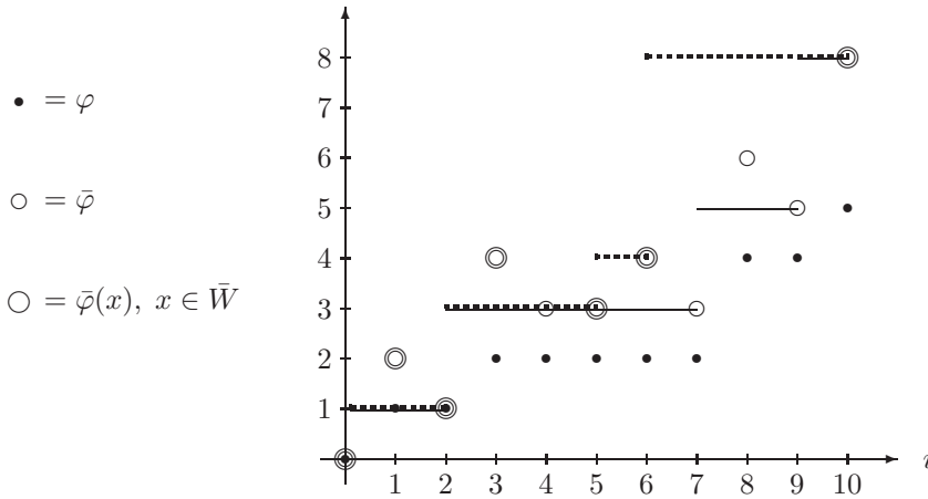
FIG. 4. Constructing \bar{W} and \tilde{\varphi} in Example 4.8.
