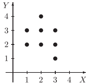
FIG. 2. X \otimes Y for X = \{1, 2, 3\} , Y(1) = \{2, 3\} , Y(2) = \{2, 3, 4\} , and Y(3) = \{1, 2, 3\} .
