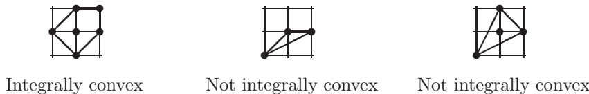
FIG. 3. Concept of integrally convex sets.
